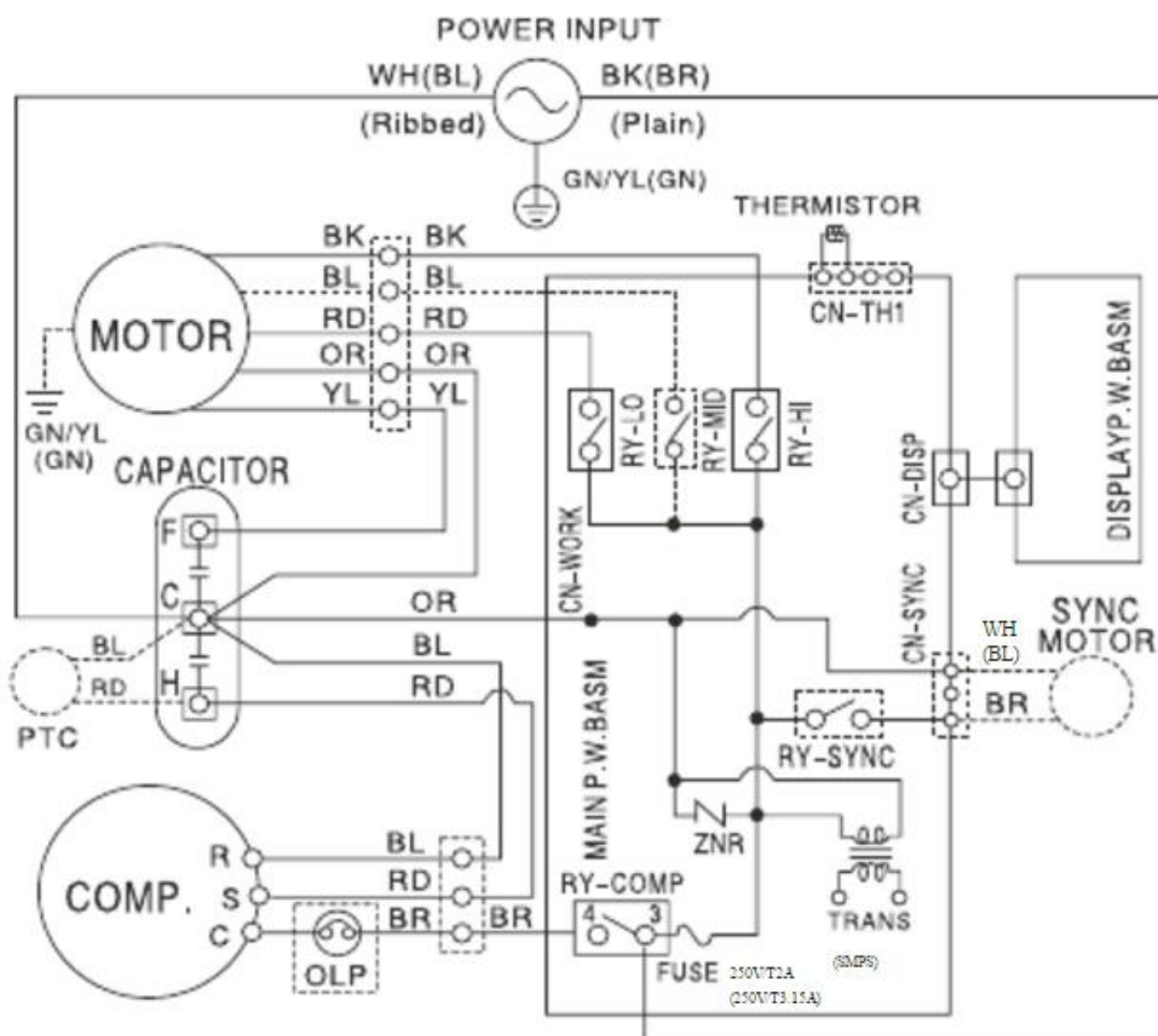
MEZ62420702 WIRING DIAGRAM
