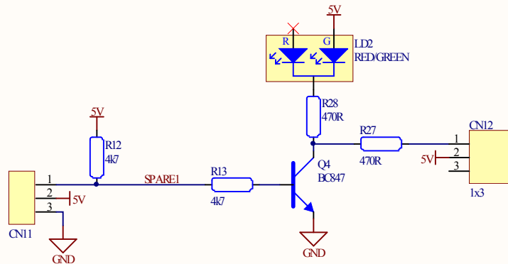
SPARE/1-WIRE/LED
